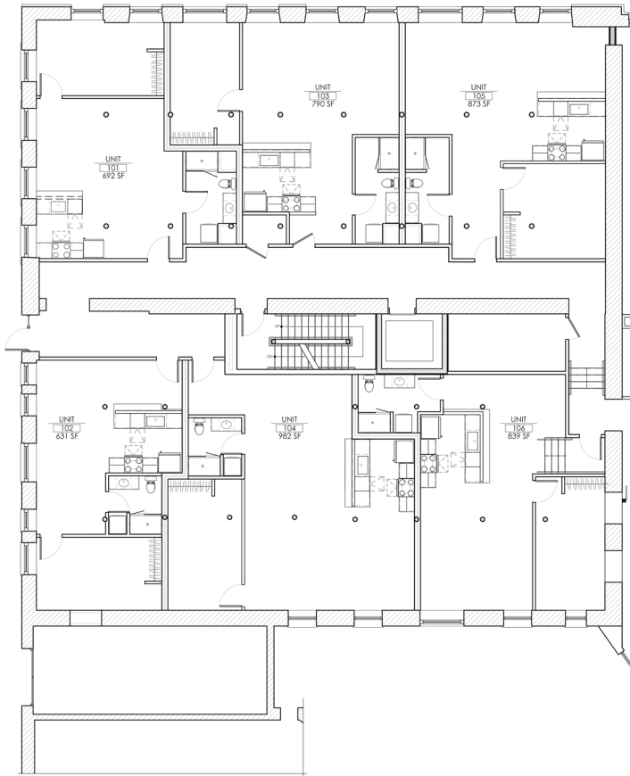
1 FIRST FLOOR PLAN SCALE: 1/8" = 1'-0"
