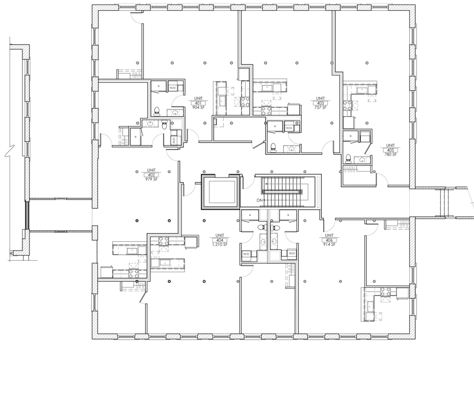
4 FOURTH FLOOR PLAN SCALE: 1/8" = 1'-0"
